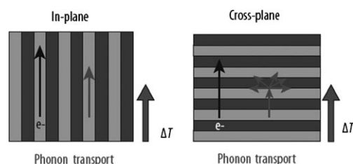
Figure 25. Mode of operation of thermoelectric multilayer structures: a) In in-plane transport, the increase in electrical conductivity owing to quantum effects dominates. b) In cross-plane transport, thermal conductivity is reduced by increased phonon scattering at the interfaces (modified reproduction of ref. [150]).
