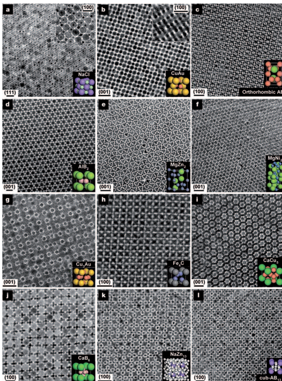
Figure 38. Cocrystallization of a) \gamma -Fe 2 O 3 and Au nanoparticles (13.4 and 5.0 nm), b) PbSe and Au nanoparticles (7.6 and 5.0 nm), c) PbSe and Pd nanoparticles (6.2 and 3.0 nm), d) PbS and Pd nanoparticles (6.7 and 3.0 nm), e) PbSe and Pd nanoparticles (6.2 and 3.0 nm), f) PbSe and Pd nanoparticles (5.8 and 3.0 nm), g) PbSe and Au nanoparticles (7.2 and 4.2 nm), h) PbSe and Pd nanoparticles (6.2 and 3.0 nm), i) PbSe and Au nanoparticles (7.2 and 5.0 nm), j) PbSe and Pd nanoparticles (5.8 and 3.0 nm), k) PbSe and Ag nanoparticles (7.2 and 4.2 nm), l) PbSe and Pd nanoparticles (6.2 and 3.0 nm) to supercrystals with various packing arrangements (scale: a–c, e, f, i–l: 20 nm; d, g, h: 10 nm; modified reproduction of ref. [297]).
