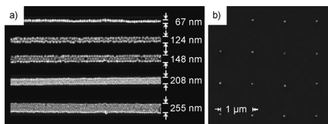
Figure 21. Printing Au nanoparticles a) as a particulate conductor path or b) as a highly ordered periodic pattern with single-particle resolution (modified reproduction of ref. [114]).
