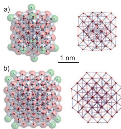
Figure 36. Structure of Ag-Se-P cluster cores in a) [Ag_{114}Se_{34}(SeiBu)_{46}(PtBu_3)_{14}] and b) [Ag_{172}Se_{40}(SenBu)_{92}(dppp)_4] with the corresponding Se sublattices (Ag blue, Se red, P green, modified reproduction of ref. [282b]).
