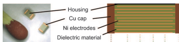
Figure 7. Photograph and schematic depiction of thin-film capacitors, which are composed in alternating layers of 200 electrodes (e.g. Ni) and 200 dielectric layers (e.g. \text{BaTiO}_3 ).
