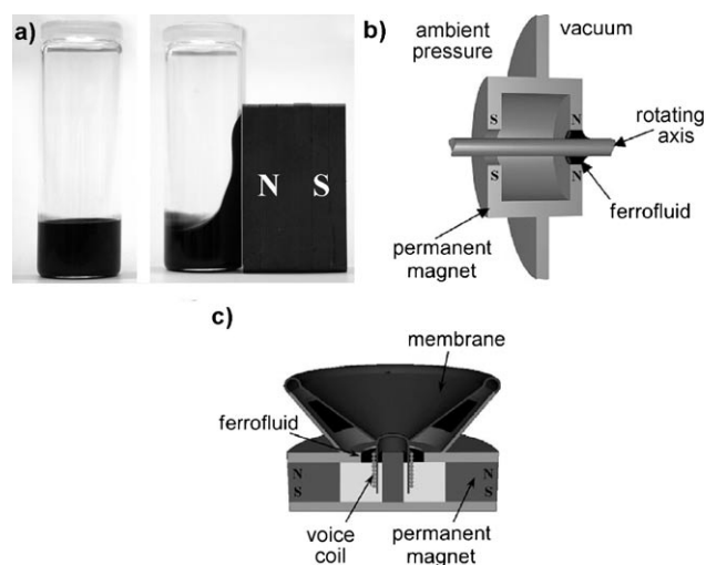
Figure 26. a) Magnetic fluid and b,c) applications as a seal around a rotating shaft (b) and as coolant in a loudspeaker (c) (modified reproduction of (a) and (b,c) from ref. [174] and [173]).
