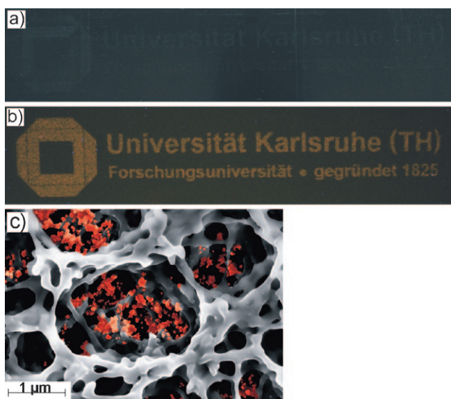
Figure 16. Transparent layer with \text{LaPO}_4\text{:Eu} nanoparticles on black cardboard a) in daylight, b) under UV light, and c) an electron microscopical image of this layer with \text{LaPO}_4\text{:Eu} nanoparticle (marked red for better visibility) between the paper fibers (modified reproduction of ref. [70]).
